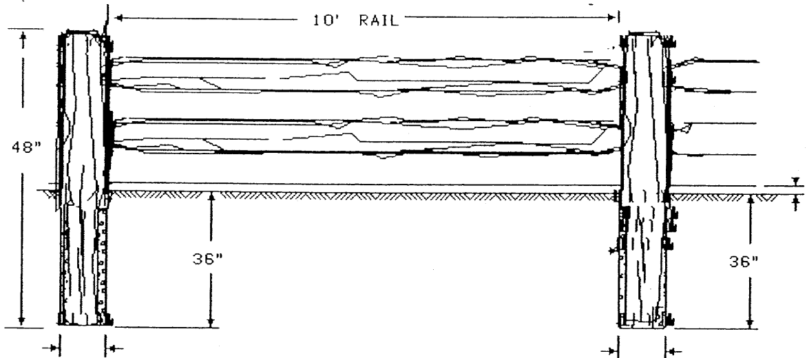
(ELEVATION VIEW)
