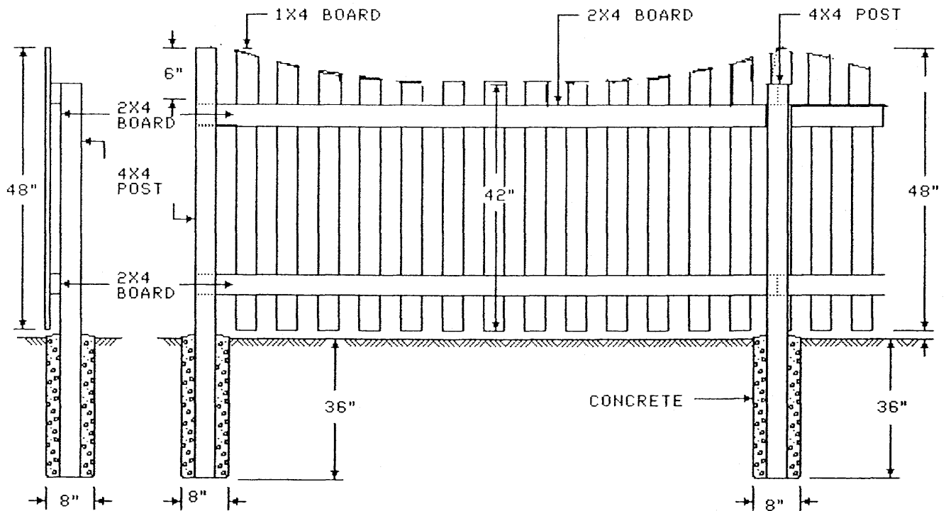
(SIDE VIEW)
