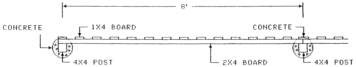
(PLAN VIEW)
